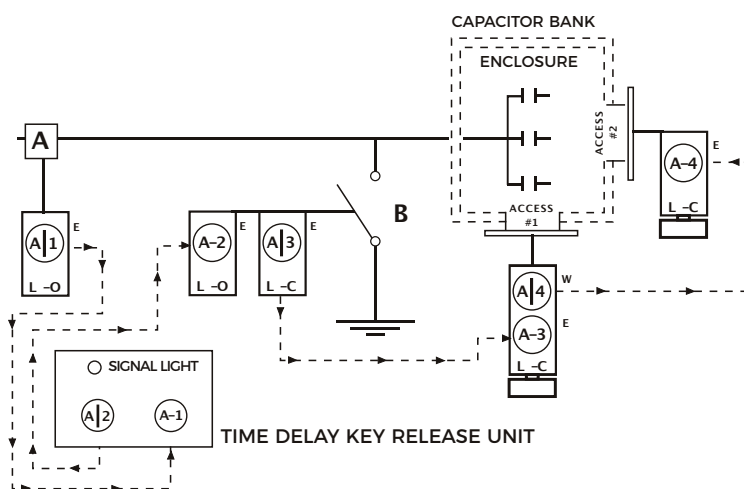
Capacitor bank scheme with time delay.
